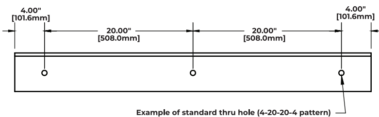
Example of standard thru hole (4-20-20-4 pattern)
